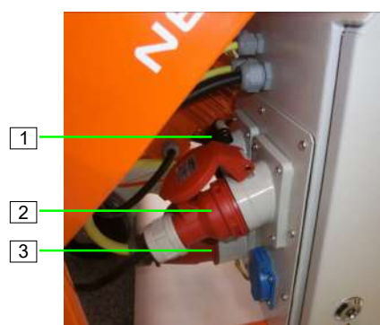
Abb. 31: Stromanschlüsse
